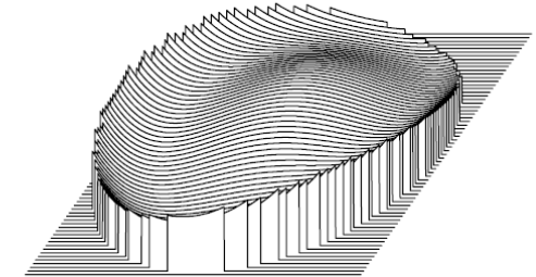
Wavefront irregularity
