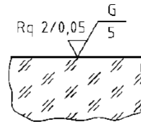
Figure 1 — Indication for ground surface with 2 \mu\text{m} > Rq > 0,05 \mu\text{m} and minimum sampling length of 5 mm
